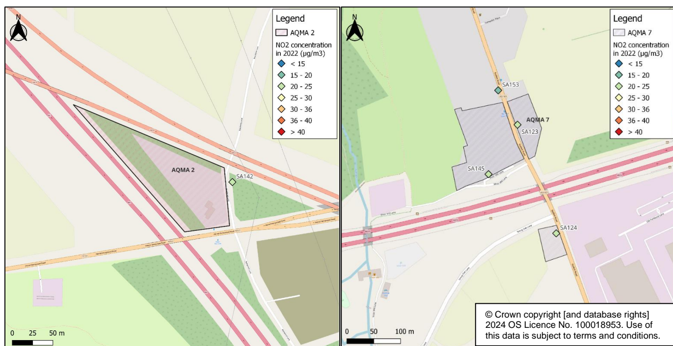
Figure 2-5: Maps of NO 2 concentrations at monitoring sites in AQMA No. 2 (left) and AQMA No. 7 (right) in St Albans City and District Council in 2022.
