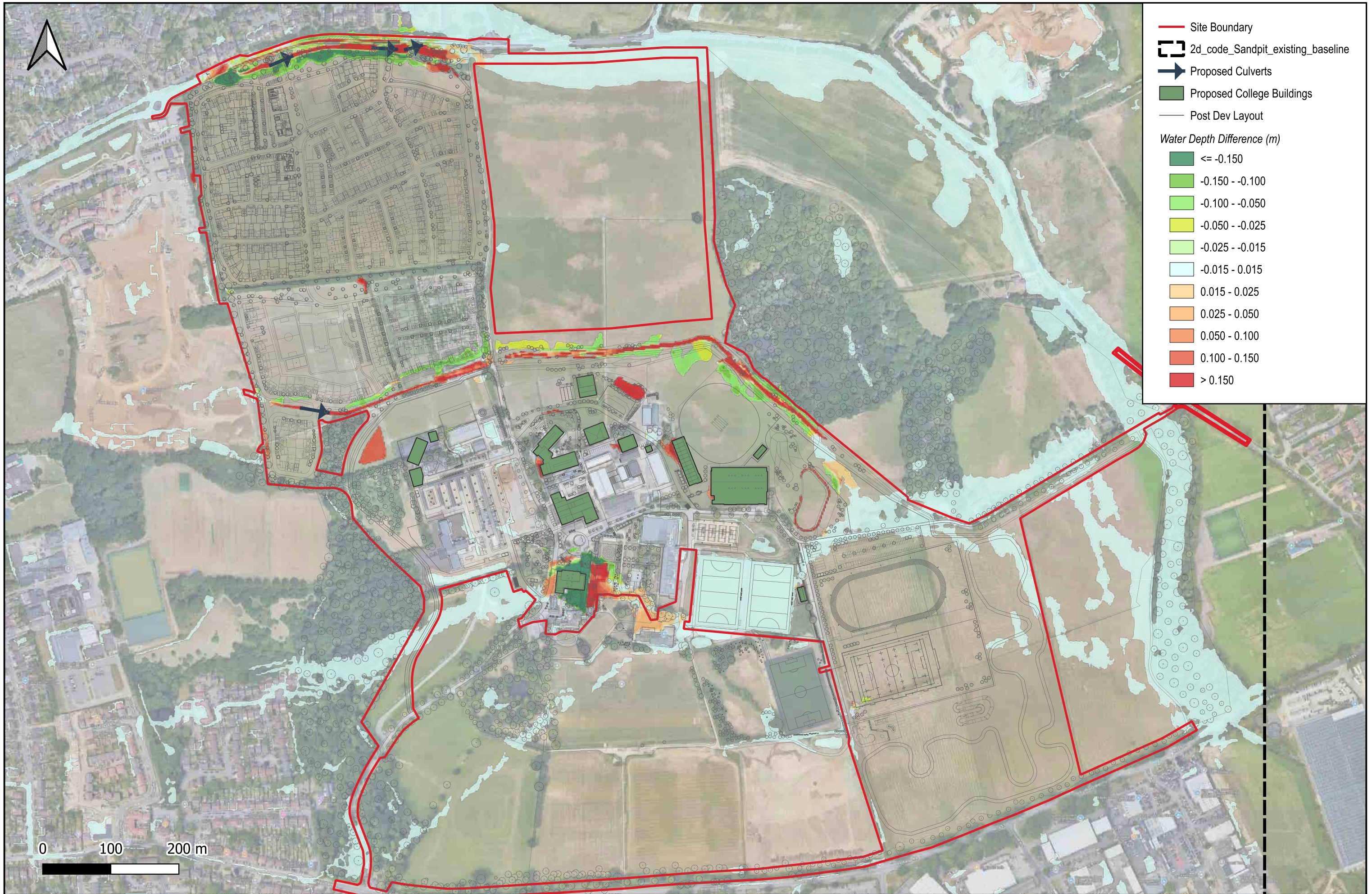
Map 14 - Sandpit Lane - Post Dev Baseline minus Existing Baseline 1hr 3.3% AEP - Comparison Depth
