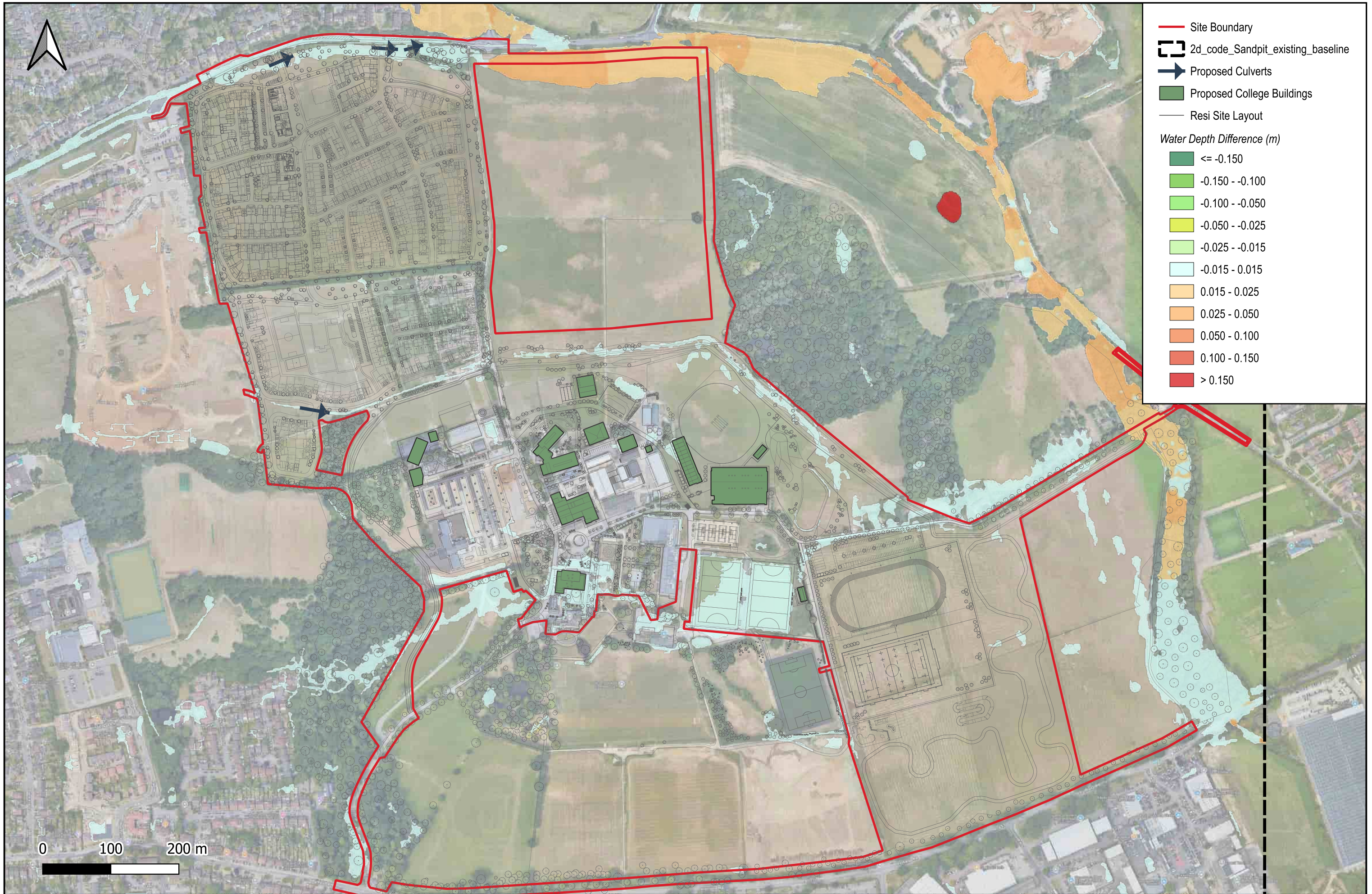
Map 17 - Sandpit Lane - Post Dev Roughness Increase minus Post Dev Baseline 1hr 1.0% AEP - Comparison Depth
