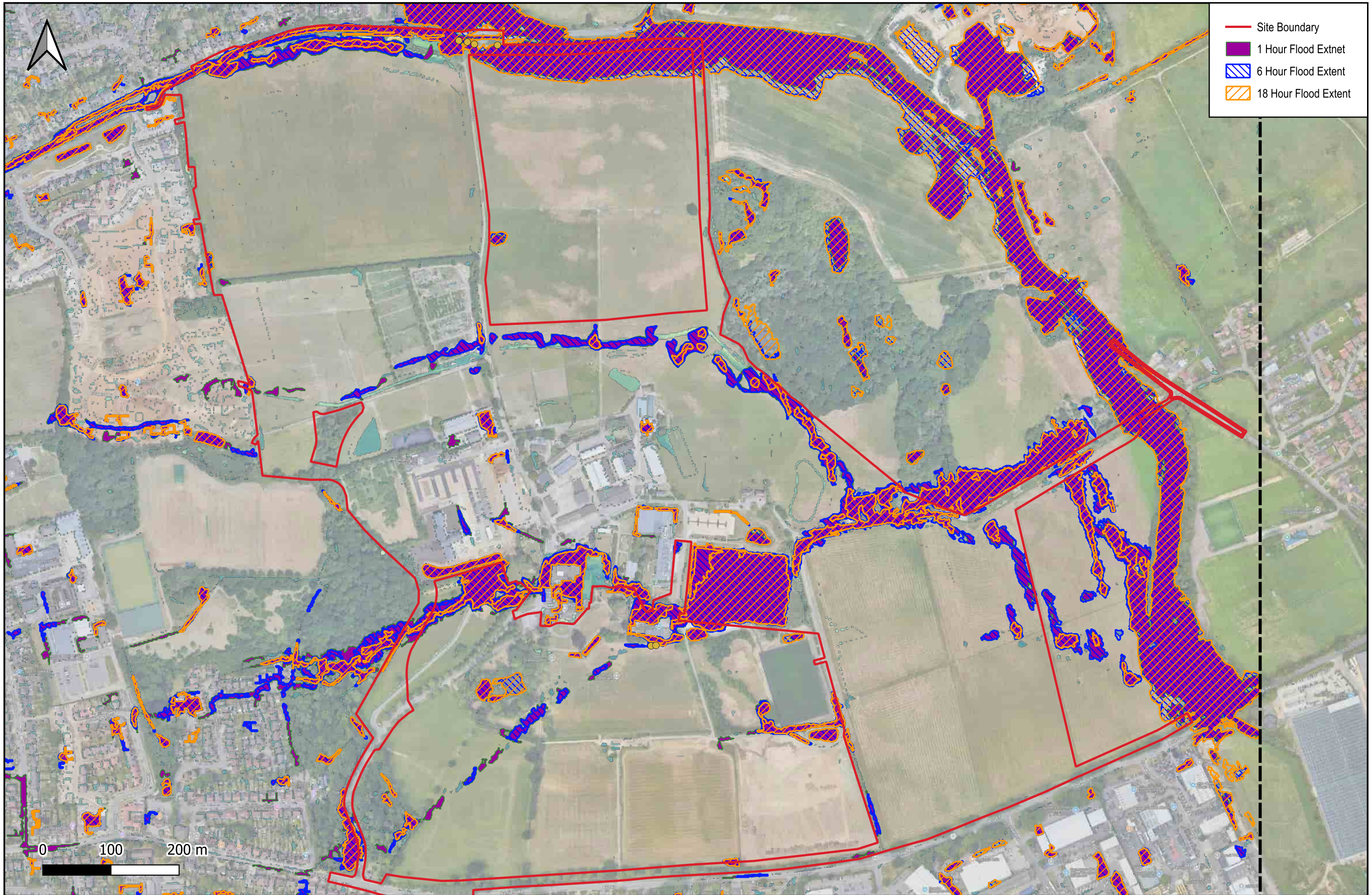
Map 20 - Sandpit Lane - Storm Duration Extents 1.0% AEP + 40%cc - 1, 6, 18 hour
