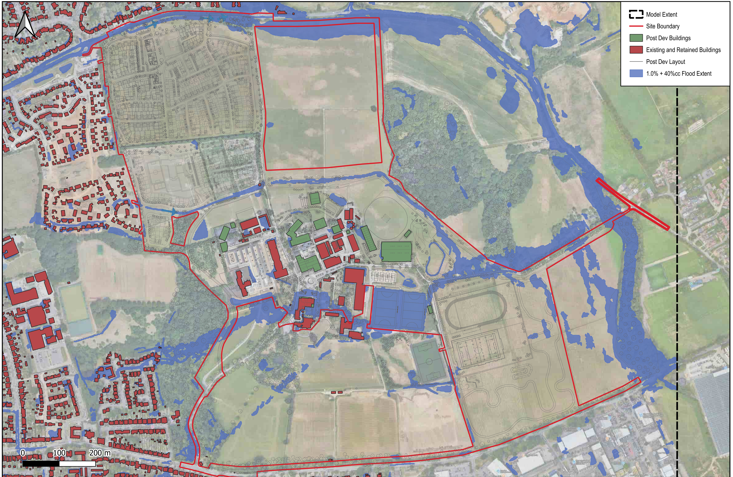
Map 21 - Sandpit Lane - Post Dev Baseline 1hr 1.0% AEP + 40% cc - Max Flood Extent
