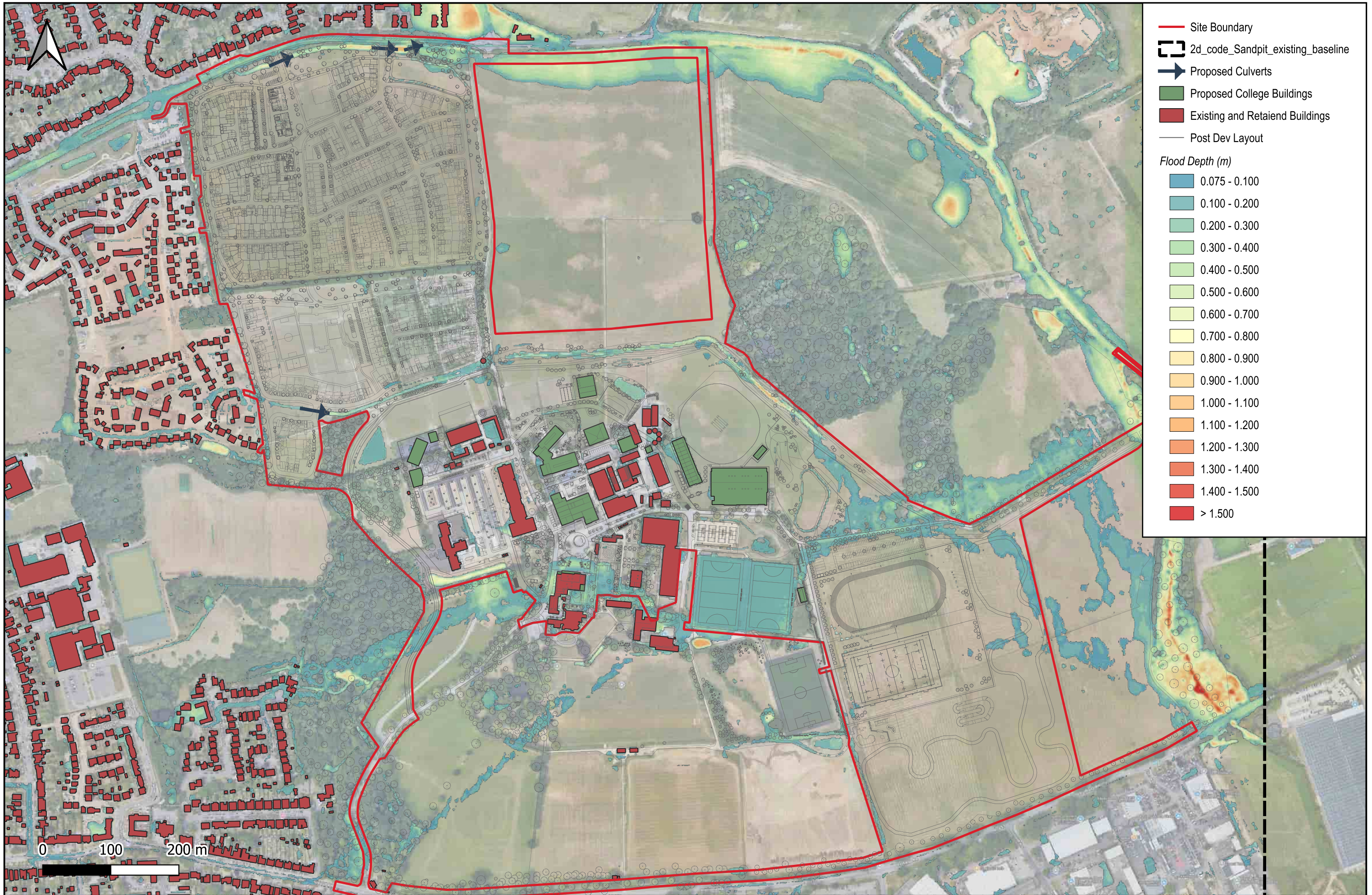
Map 08 - Sandpit Lane - Post Dev Baseline 1hr 0.1% AEP - Max Flood Depth
