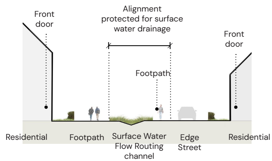
FIGURE 72 - ALIGNMENT PROTECTED FOR SURFACE WATER DRAINAGE ILLUSTRATIVE SECTION
